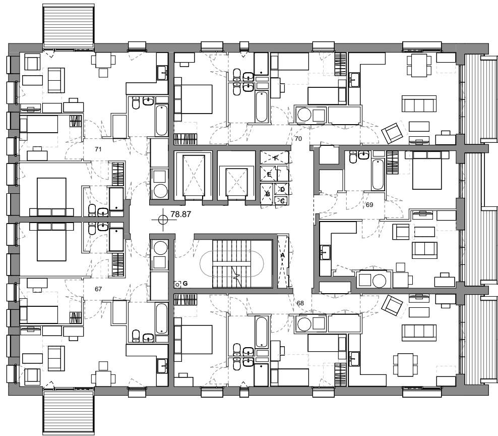
01 TENTH FLOOR PLAN
