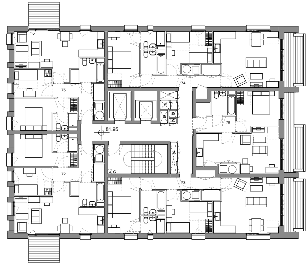
02 ELEVENTH FLOOR PLAN
