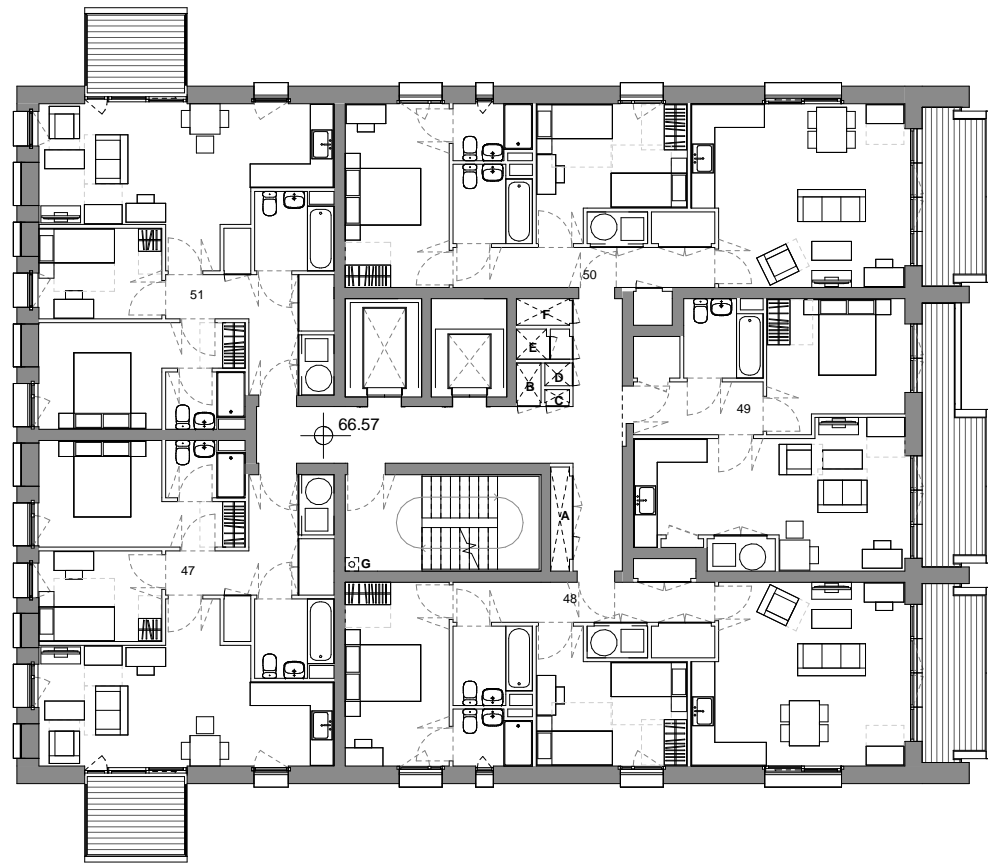
01 SIXTH FLOOR PLAN
