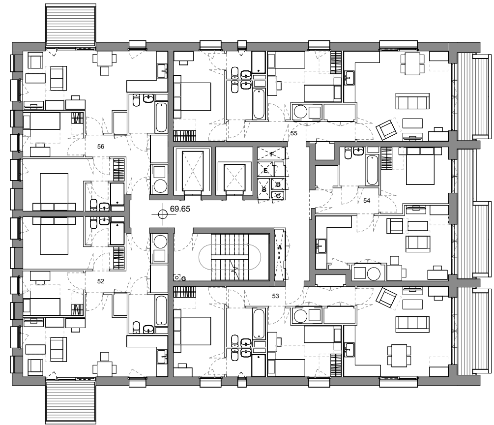
02 SEVENTH FLOOR PLAN
