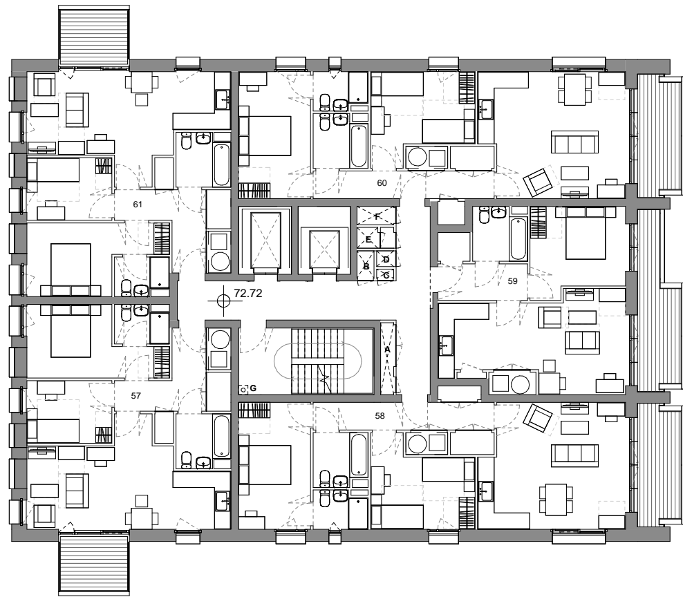
01 EIGHTH FLOOR PLAN
