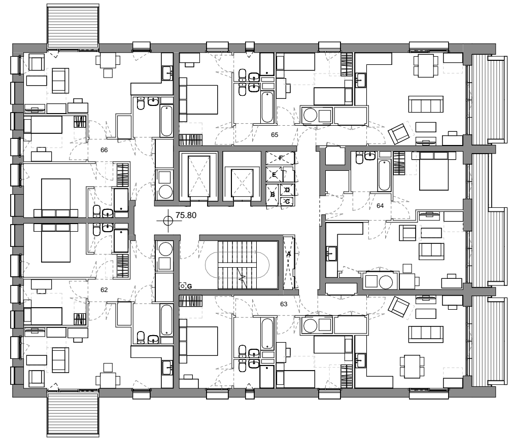
02 NINTH FLOOR PLAN
