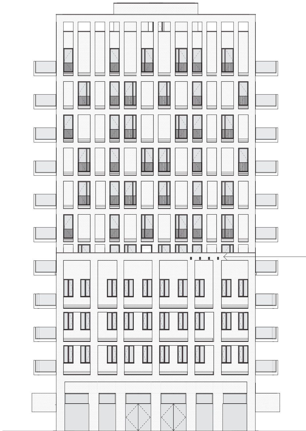
North-East Elevation bird box location 1:200
